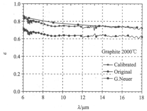
图 10 石墨在 2000℃的发射率校正结果与文献数据对比 Fig. 10 The comparison of calibrated graphite emissivity results and reference data at 2000℃
