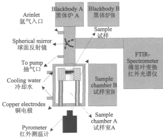
图 1 超高温光谱发射率测量原理图 Fig 1 Schematic diagram of ultra-high temperature spectral emissivity measurement
