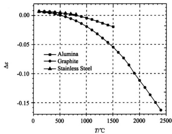
图 7 3 种试样在各温度的发射率测量偏差 Fig 7 Emissivity deviation of three samples at different temperature
