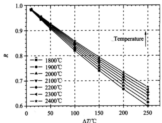
图 3 温度测量偏差引起发射率测量结果衰减比 Fig 3 Attenuation ratio of emissivity results caused by temperature measurement deviation
