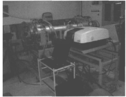
图 2 课题组研制的发射率测量系统 Fig 2 Emissivity measurement system developed by research team
