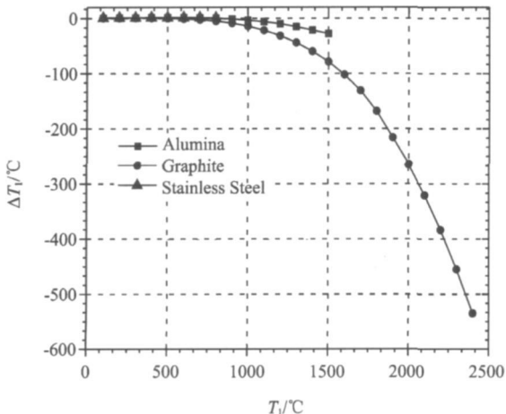
图 6 热平衡状态时试样真温与测量温差的关系 Fig 6 The relationship between sample temperature and measurement temperature difference at thermal balance
