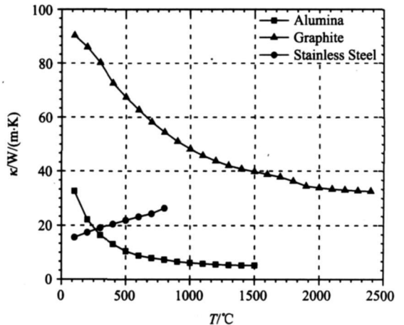
图 5 材料热导率与温度的关系曲线图 Fig 5 The relationship between material thermal conductivity and temperature
