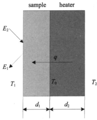
图 4 试样辐射和一维热传导模型 Fig 4 Sample radiation and one-dimensional heat transfer model
