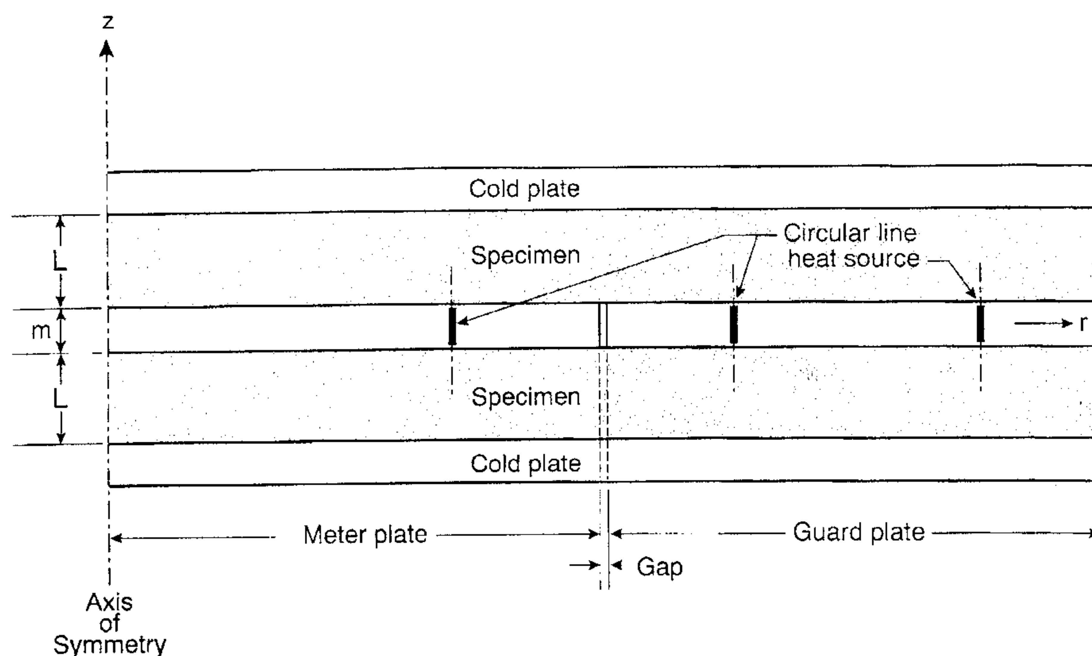
FIG. 1 Schematic of a Line-Heat-Source Guarded-Hot-Plate Apparatus
