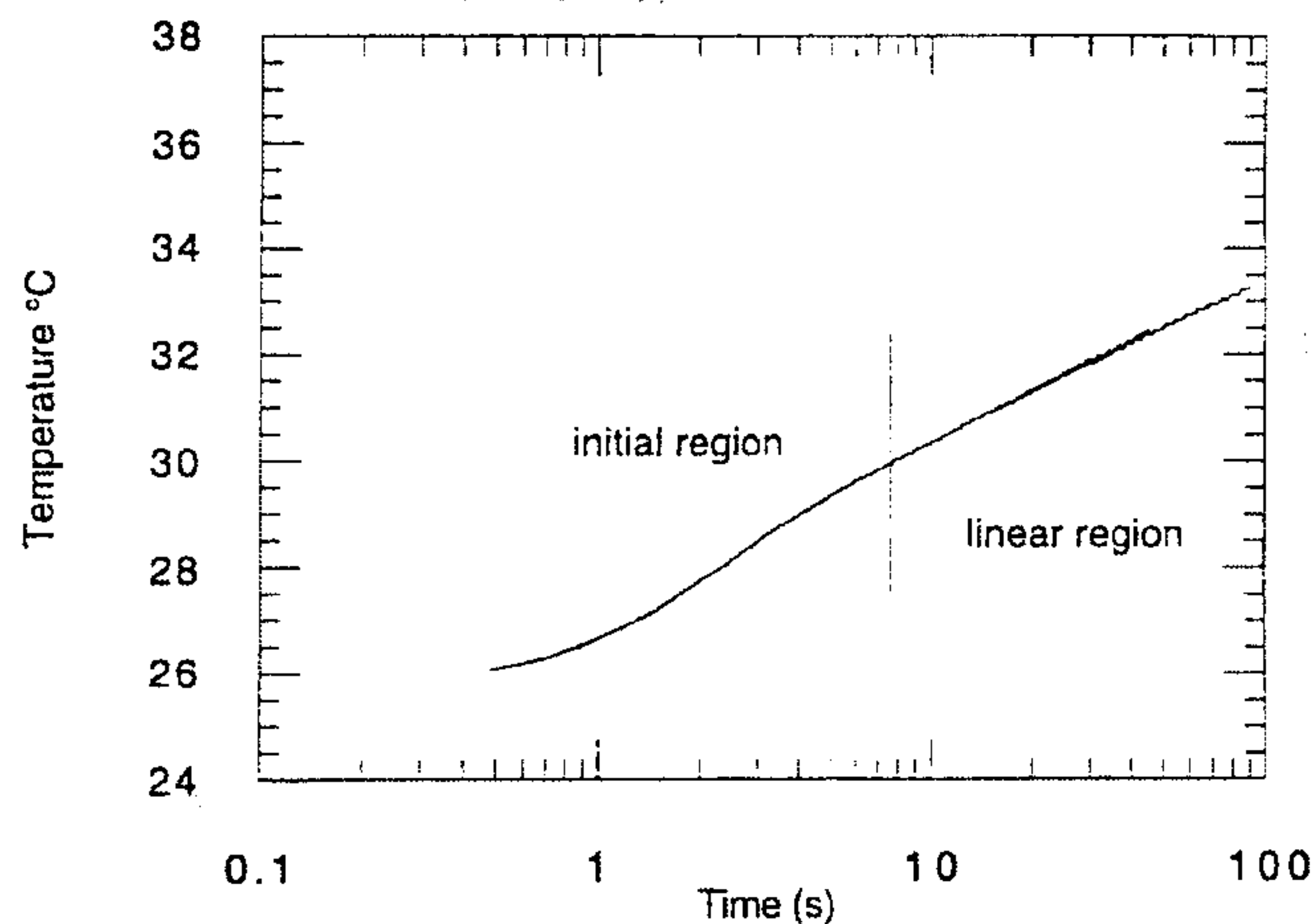
FIG. 1 Line-Source Transient
