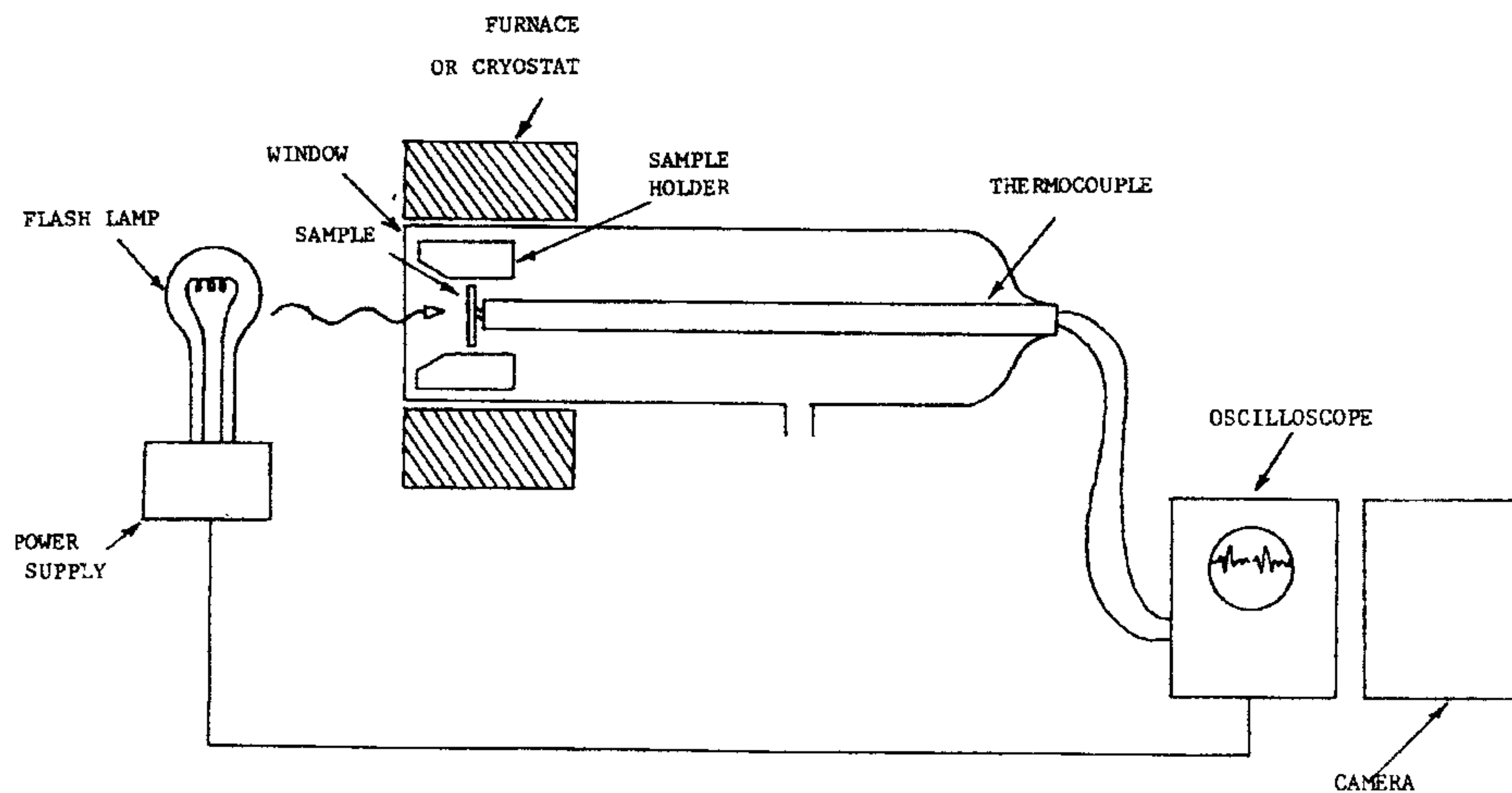
FIG. 3 Schematic Diagram of Apparatus
