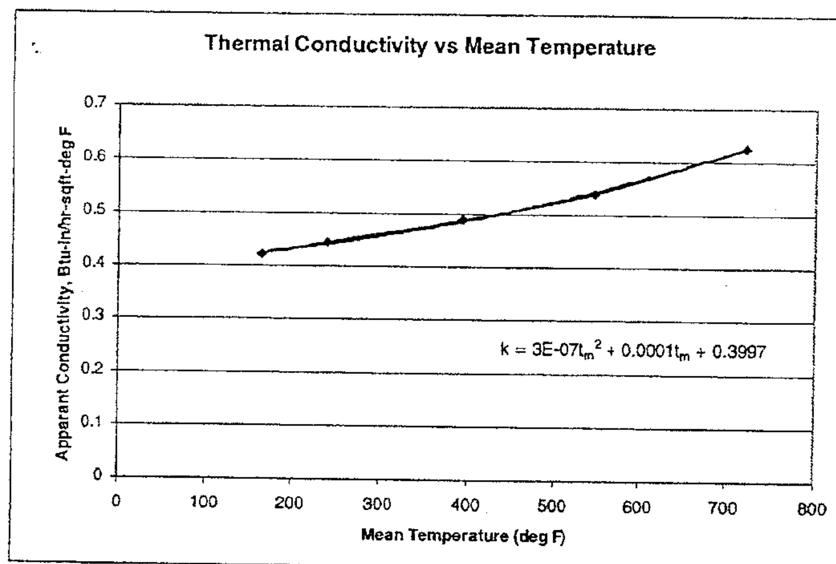
FIG. 3 Mean Temperature vs. Thermal Conductivity
