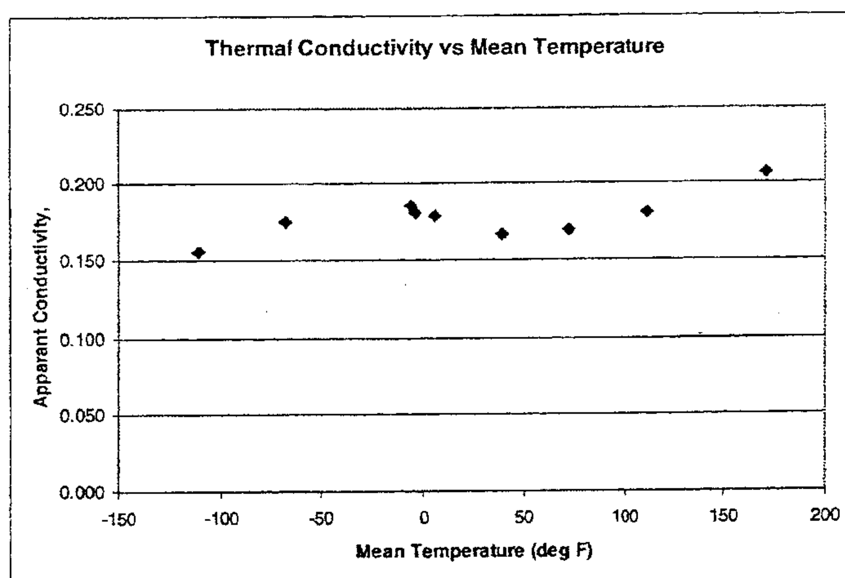
FIG. 4 Thermal Conductivity vs. Mean Temperature
