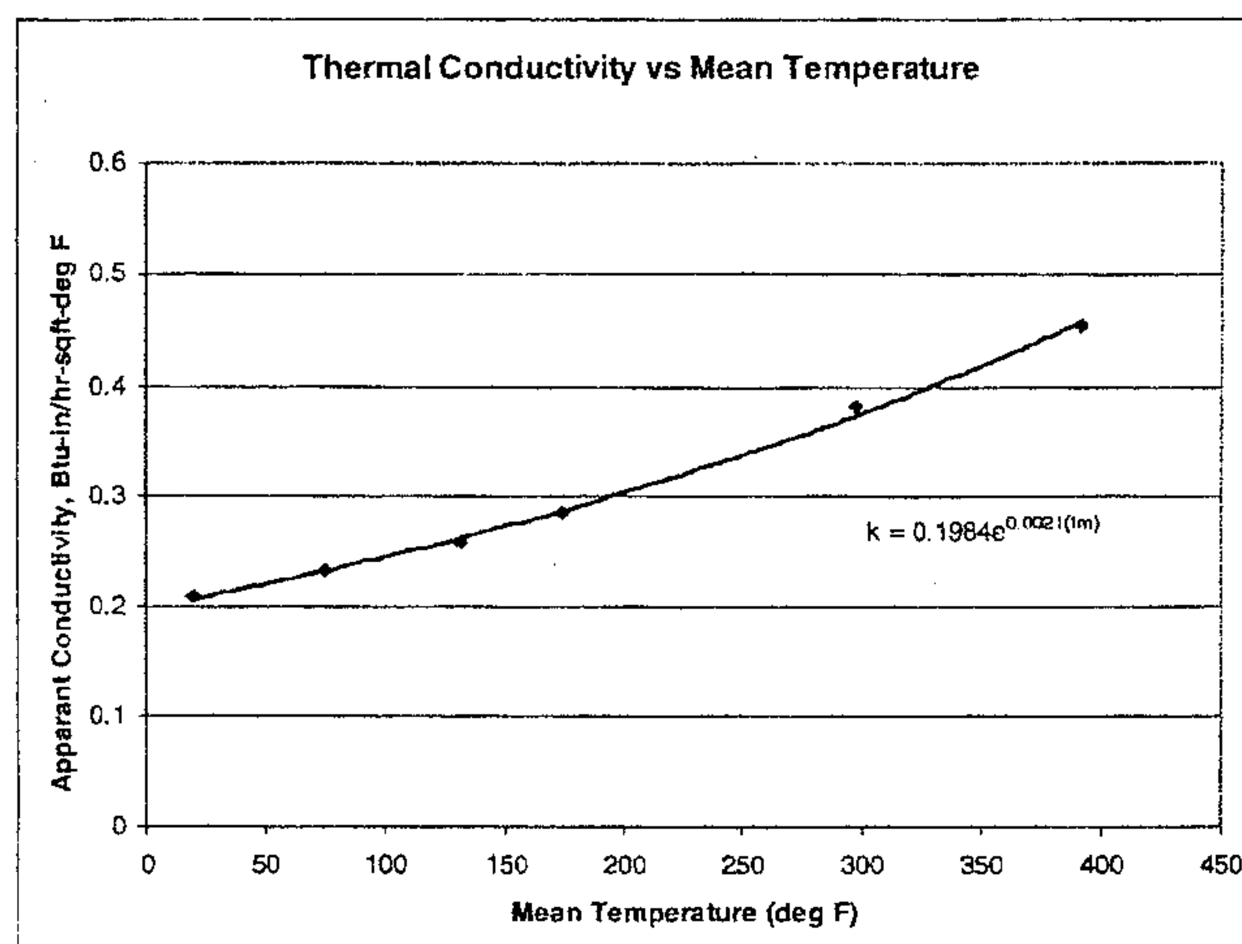
FIG. 2 Thermal Conductivity vs. Mean Temperature
