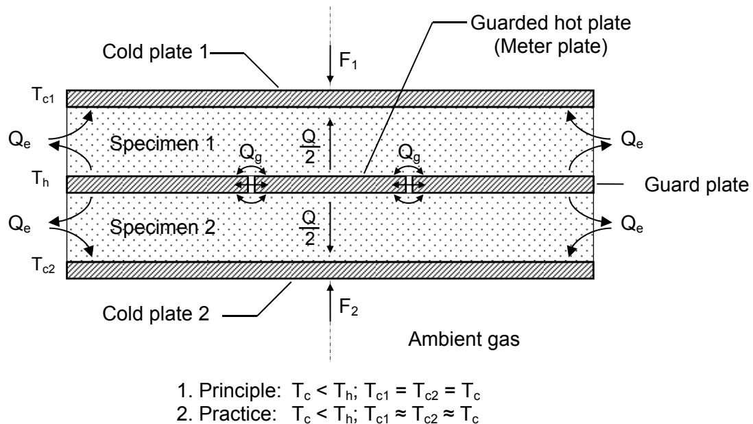
Figure 8. Guarded-hot-plate schematic (not to scale) showing the double-sided mode of operation with vertical heat flow.
