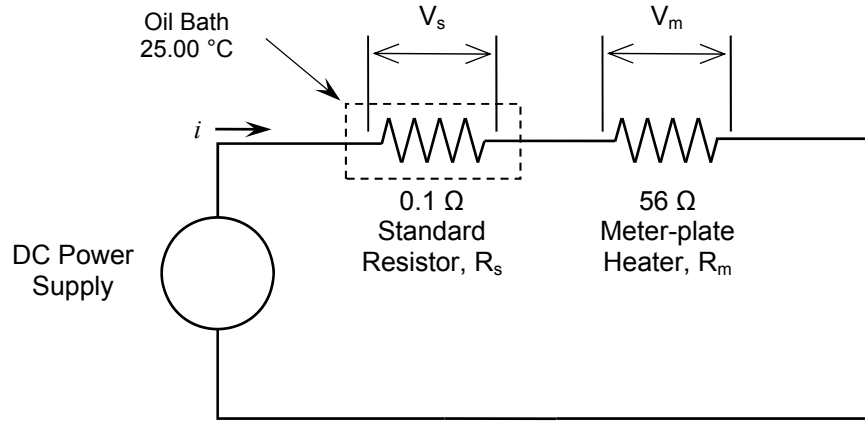
Figure A1. Electrical schematic for meter-plate power measurement.
