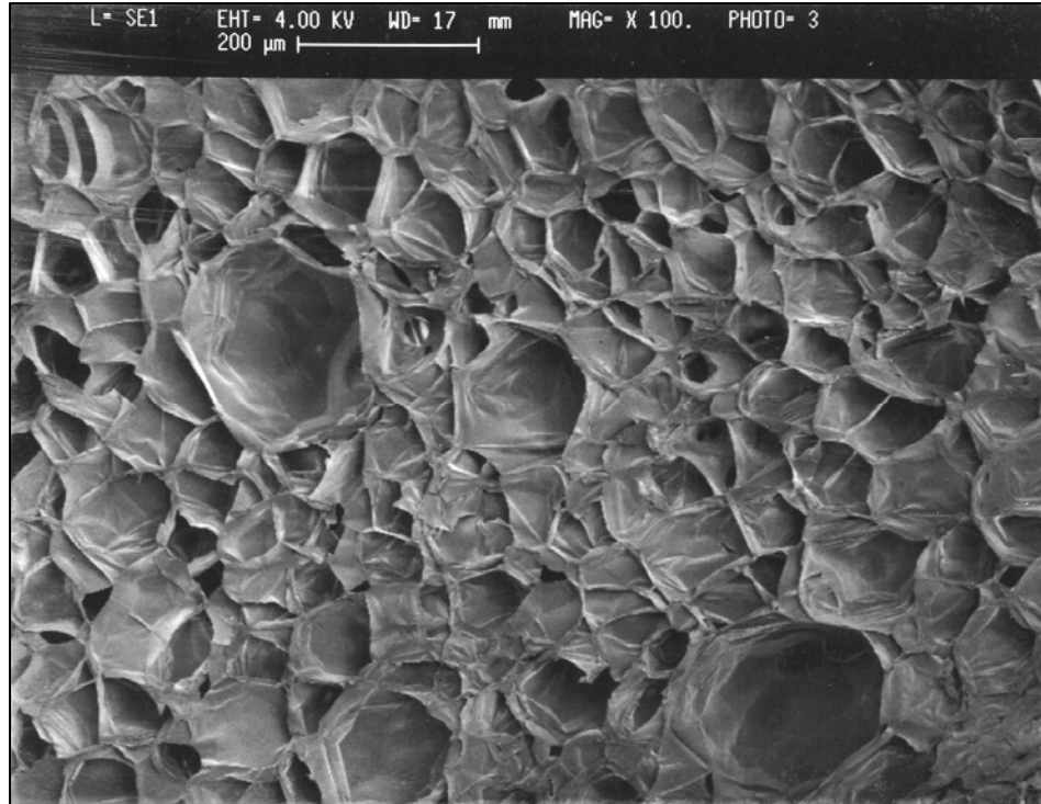
Figure 7b. SEM micrograph (100 \times ) shows close-up of cellular structure
