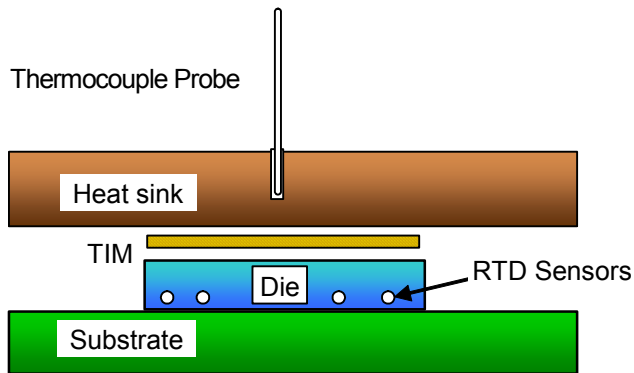
Figure 2: Schematic of TIM thermal test vehicle.
