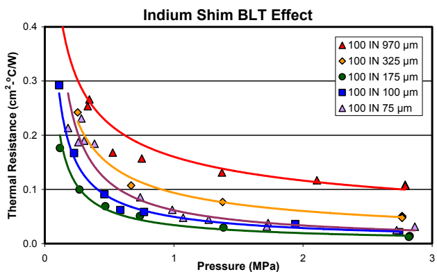
Figure 4: Plots of thermal resistance of indium shim of different thicknesses.
