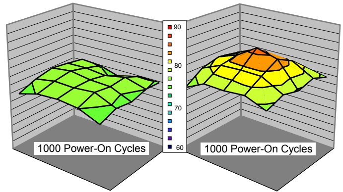
Figure 7: Temperature profiles of TIM materials subjected to power cycling. The thermal grease pump-out profile is shown on the right in contrast to a stable metal TIM on the left.
