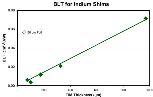
Figure 6: BLT thermal resistance contribution for the indium metal TIM.
