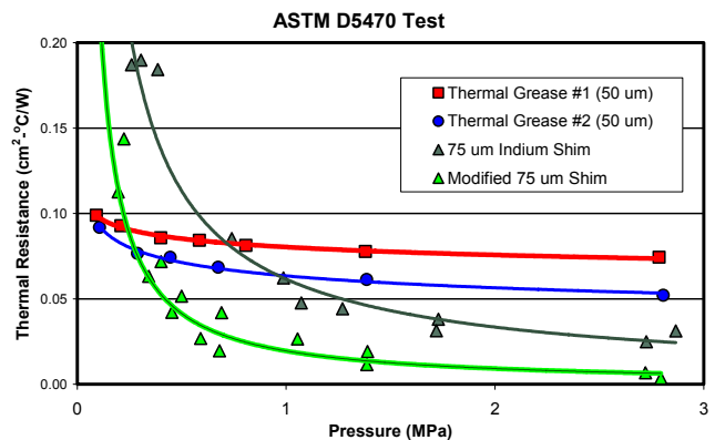
Figure 3: Plot of the thermal resistance of several TIM materials as a function of applied clamping pressure.
