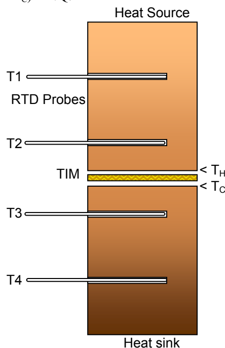
Figure 1: Schematic of TIM and test block configuration of ASTM D5470 tester.
