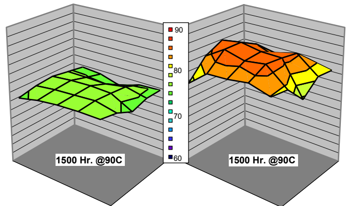
Figure 8: Temperature profiles of TIM materials after thermal exposure. The bake-out profile of grease is shown on the right in contrast to a stable metal TIM on the left.
