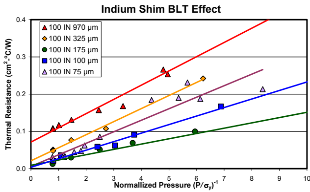
Figure 5: Plot showing the relationship thermal resistance vs. the inverse of pressure.
