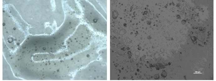
Figure 6: Grease drop on PET before thermal testing (left), Residues of soldering grease on bare PET after thermal testing and cleaning (right)
