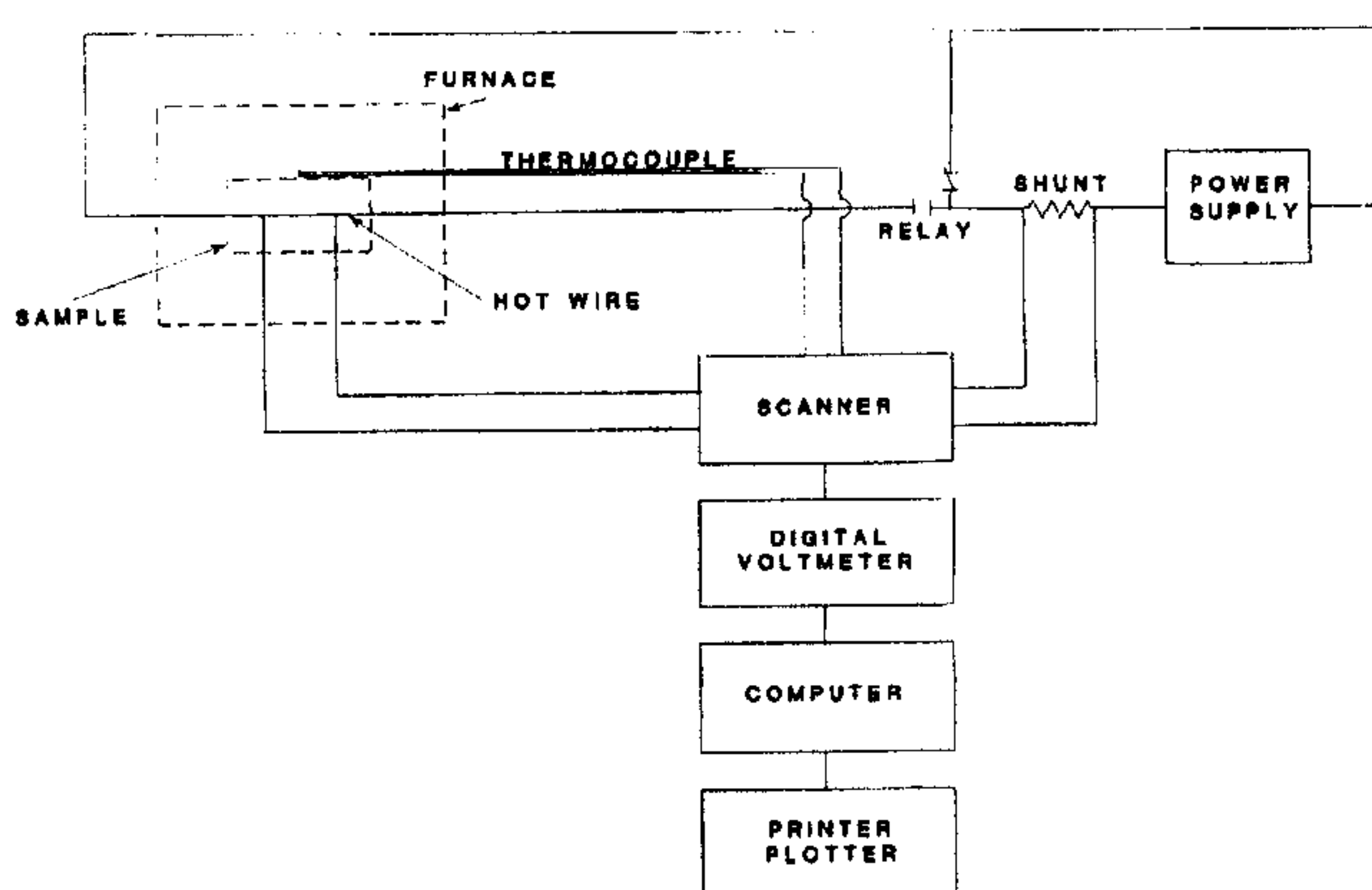
FIG. 1 Diagram of Apparatus
