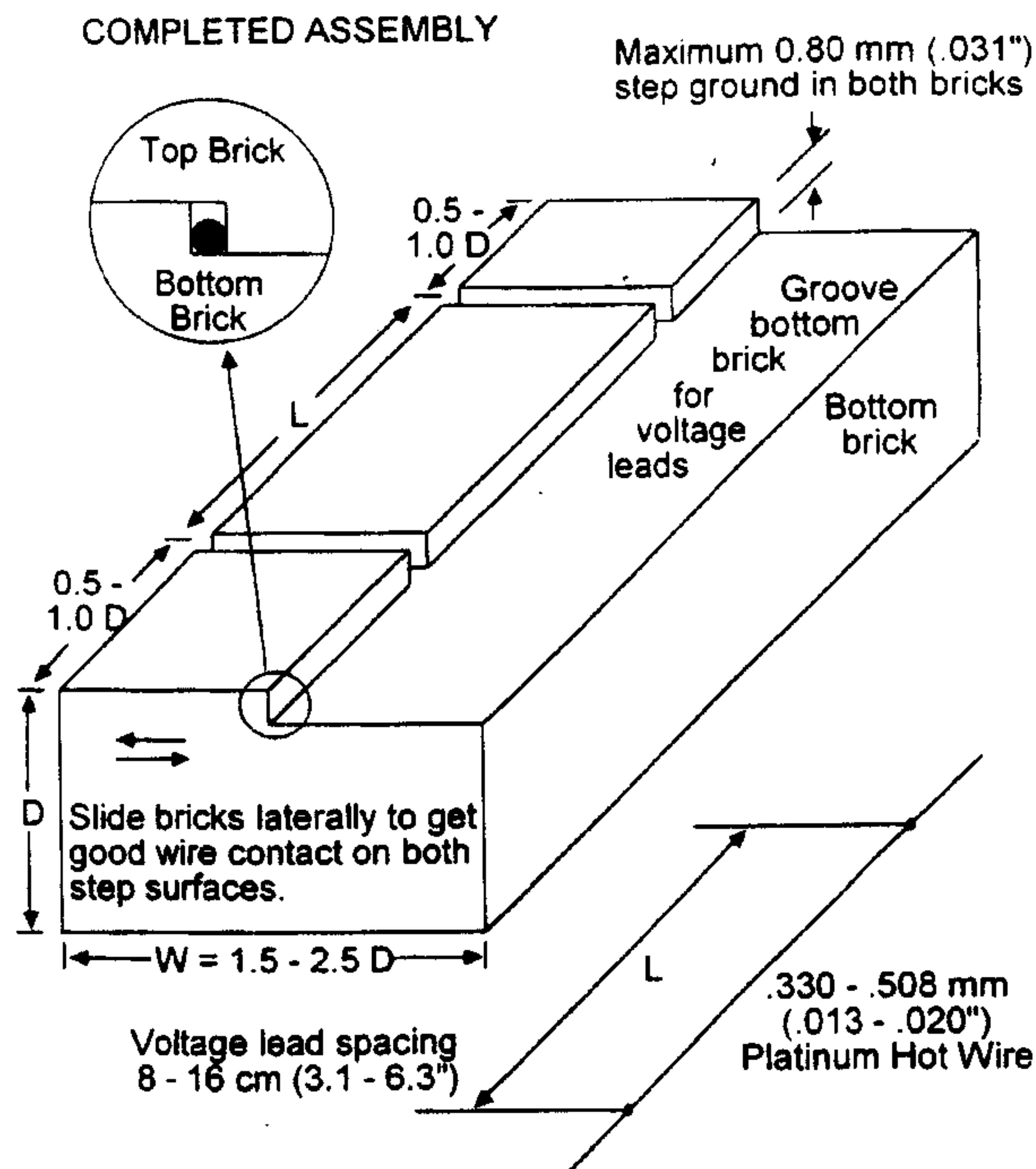
FIG. 2 Hot Wire Sample Setup
