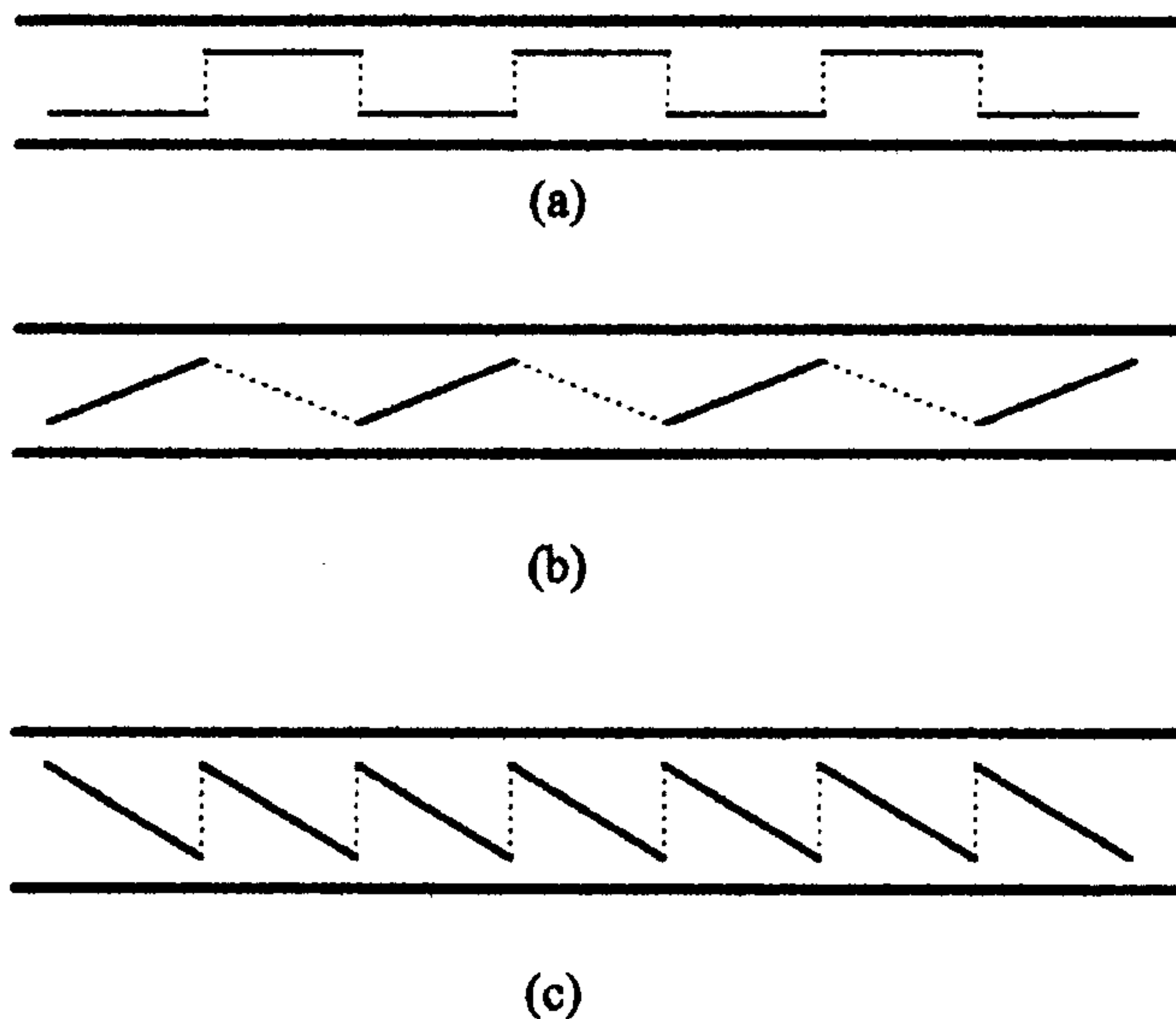
FIG. X1.2 Schematic Designs of Transducers
