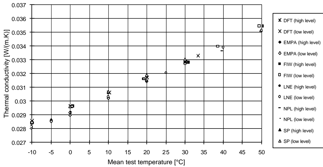
Figure A5b: Thermal conductivity versus temperature over the range [-10 ^{\circ}C / + 50 ^{\circ}C ]
