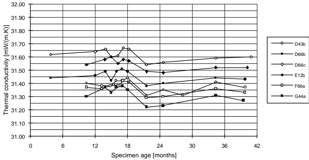
Figure A3: Thermal conductivity versus specimen age
