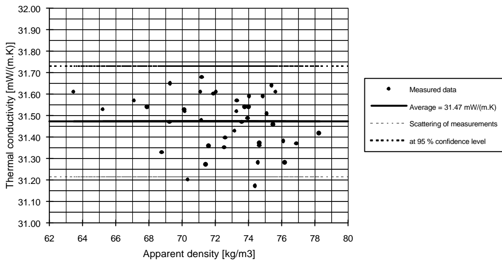
Figure A2k: Thermal conductivity versus specimen density
