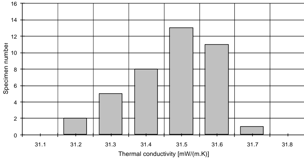
Figure A2i: Histogram of thermal conductivity distribution
