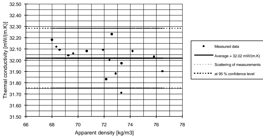
Figure A2j: Thermal conductivity versus specimen density
