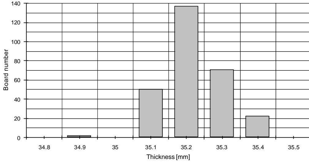
Figure A1a : Histogram of board thickness distribution
