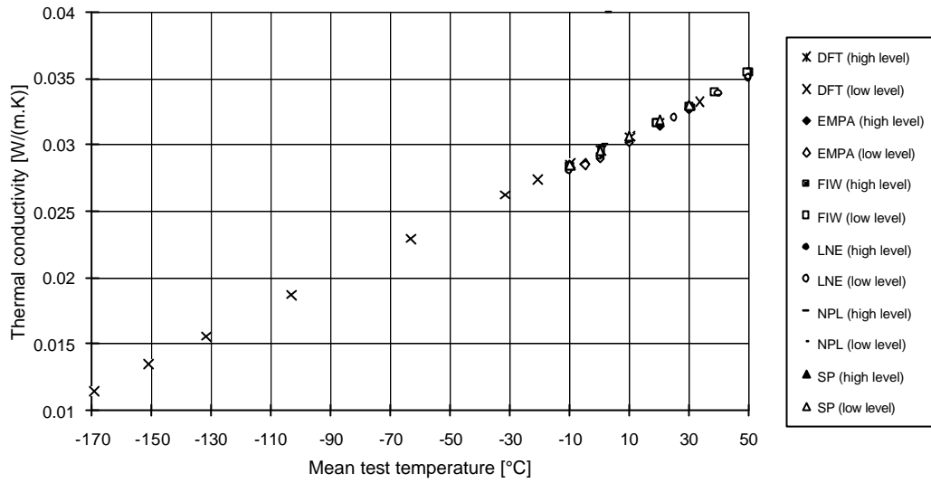
Figure A5a: Thermal conductivity versus temperature over the range [-170 ^{\circ}C / + 50 ^{\circ}C ]
