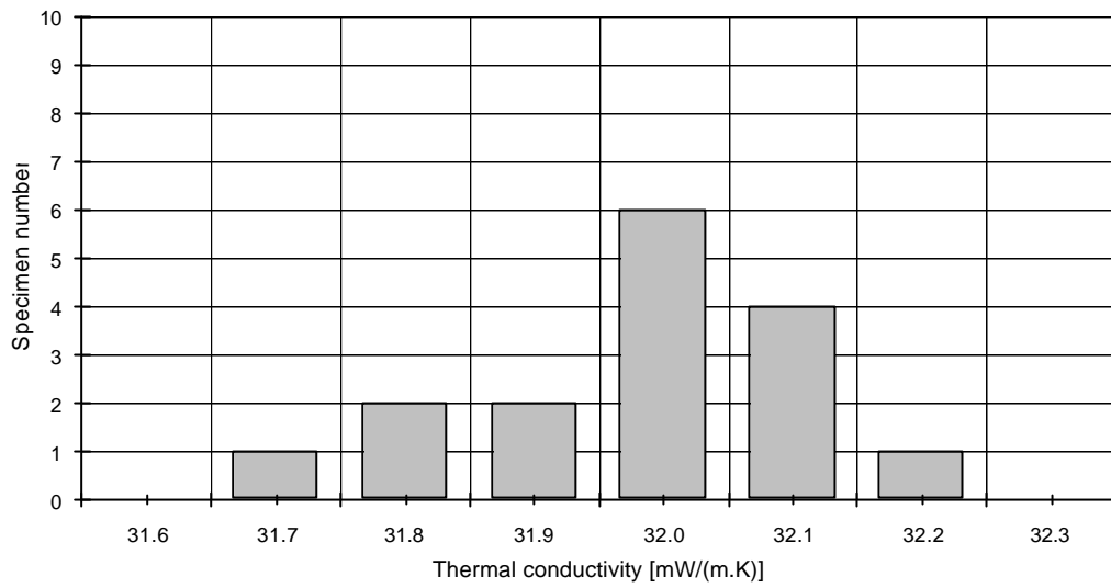
Figure A2h: Histogram of thermal conductivity distribution
