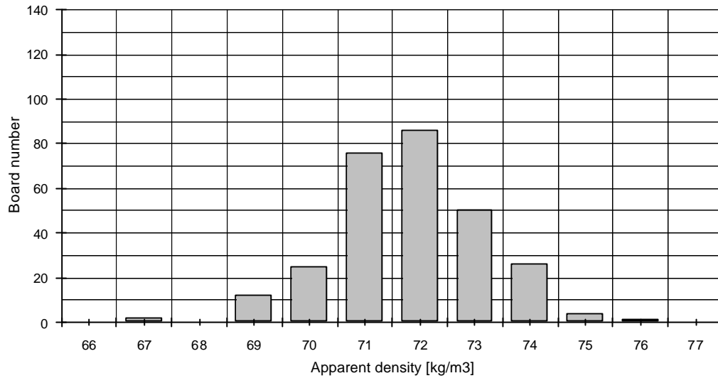
Figure A1c : Histogram of board density distribution
