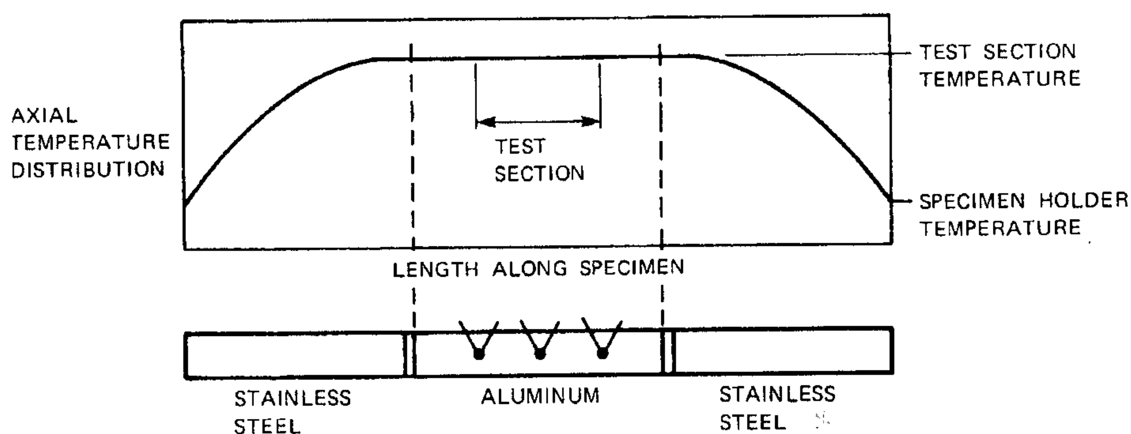
FIG. 8 Composite Specimen
