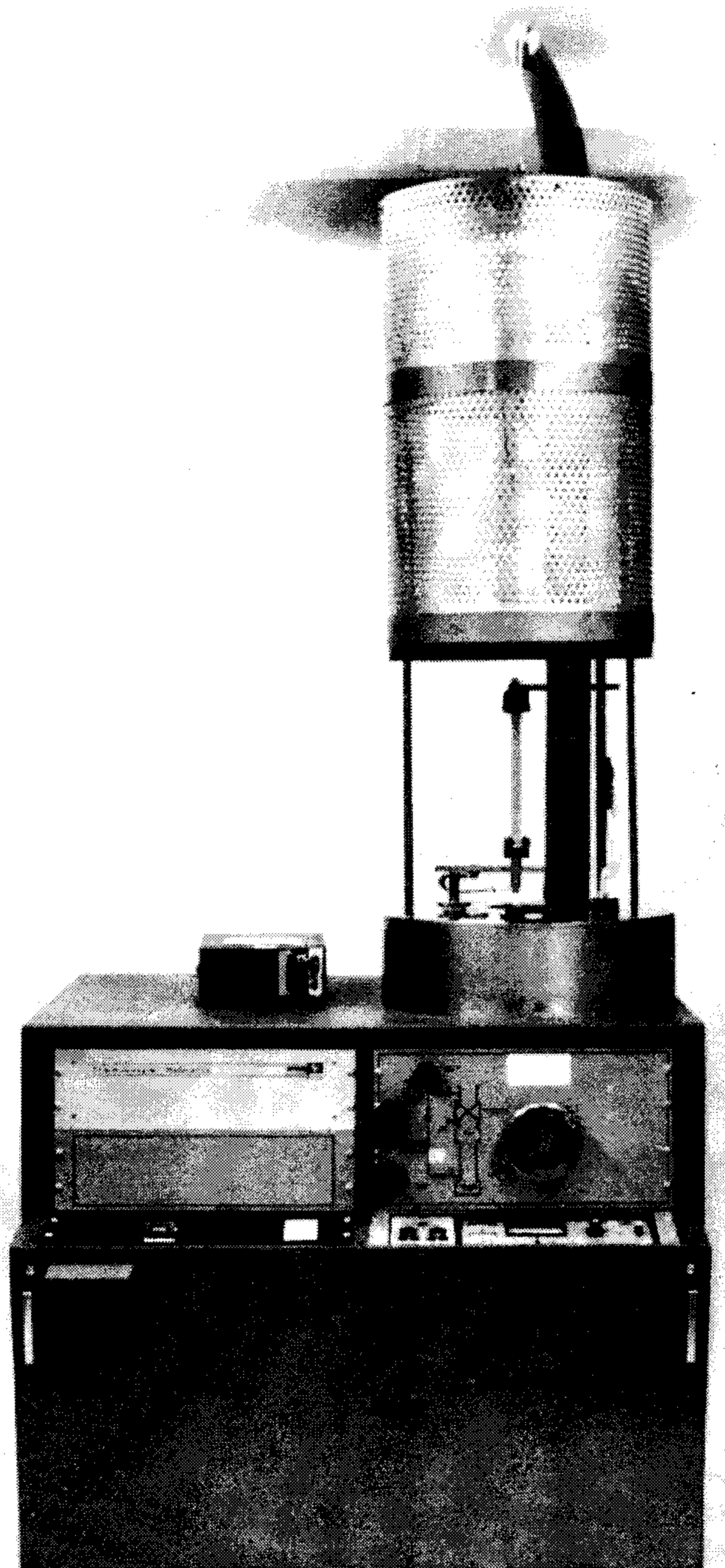
FIG. 3 Example of Vacuum Emittance Test Facility
