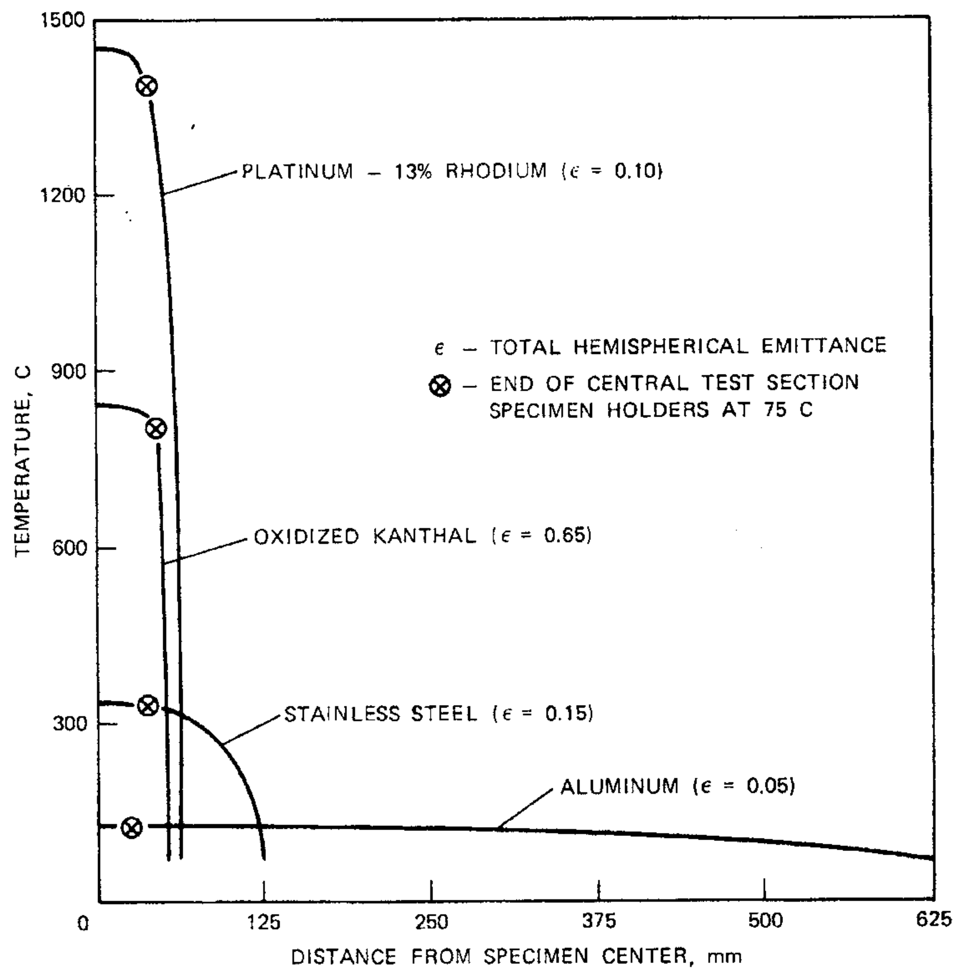
FIG. 7 Predictions of Specimen Temperature Distributions
