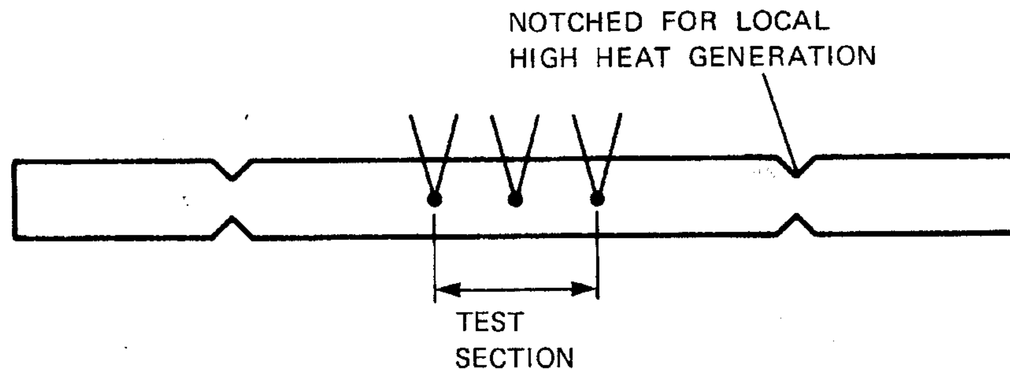
FIG. 9 Notched Specimen
