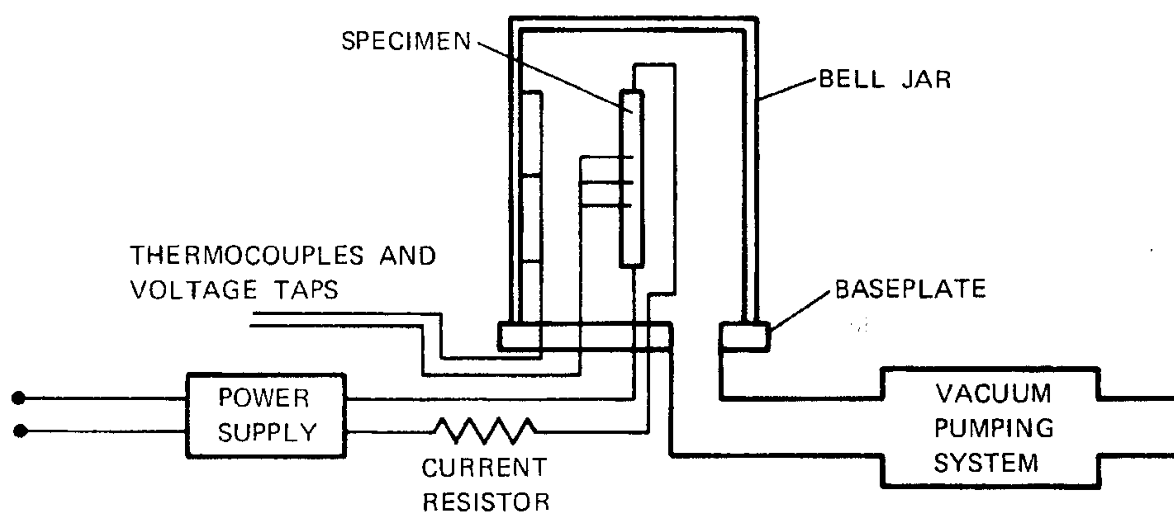
FIG. 1 System Arrangement
