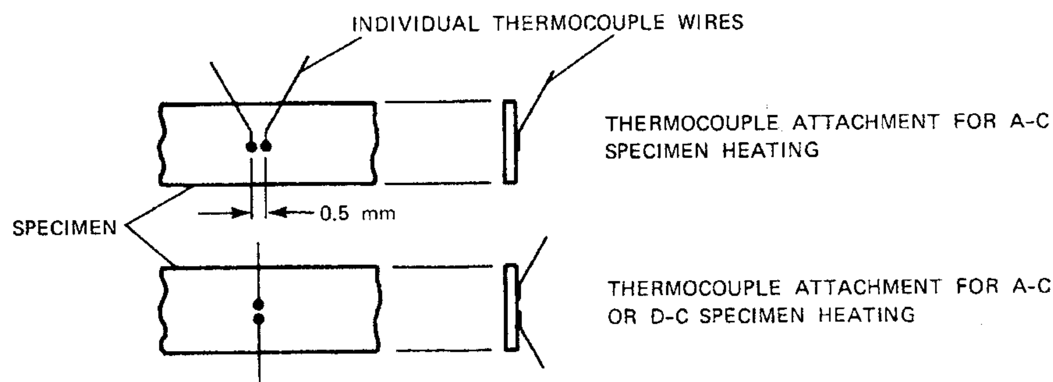
FIG. 6 Thermocouple Attachment
