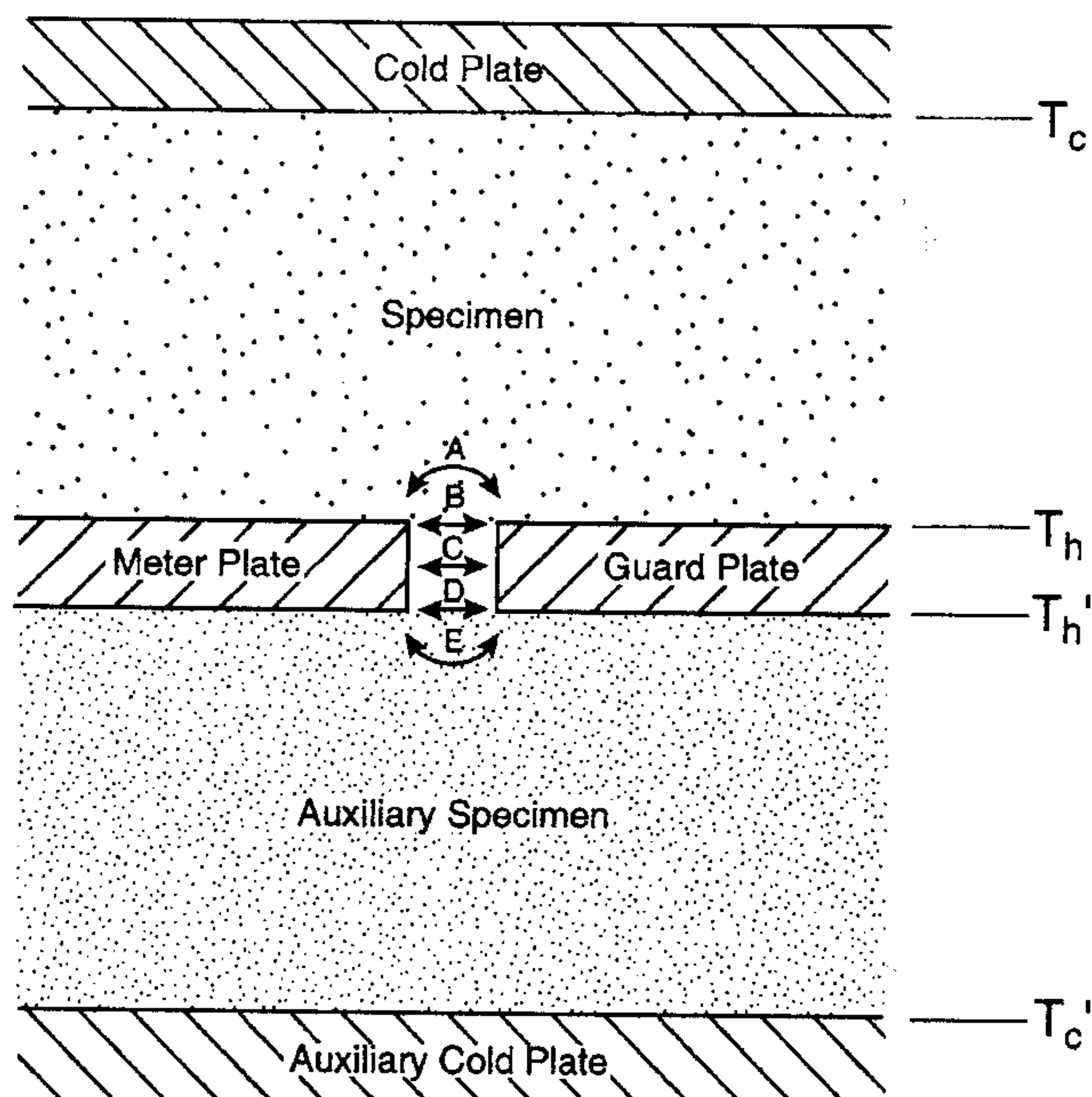
FIG. X2.1 Diagram Illustrating Heat Flows at Gap Region
