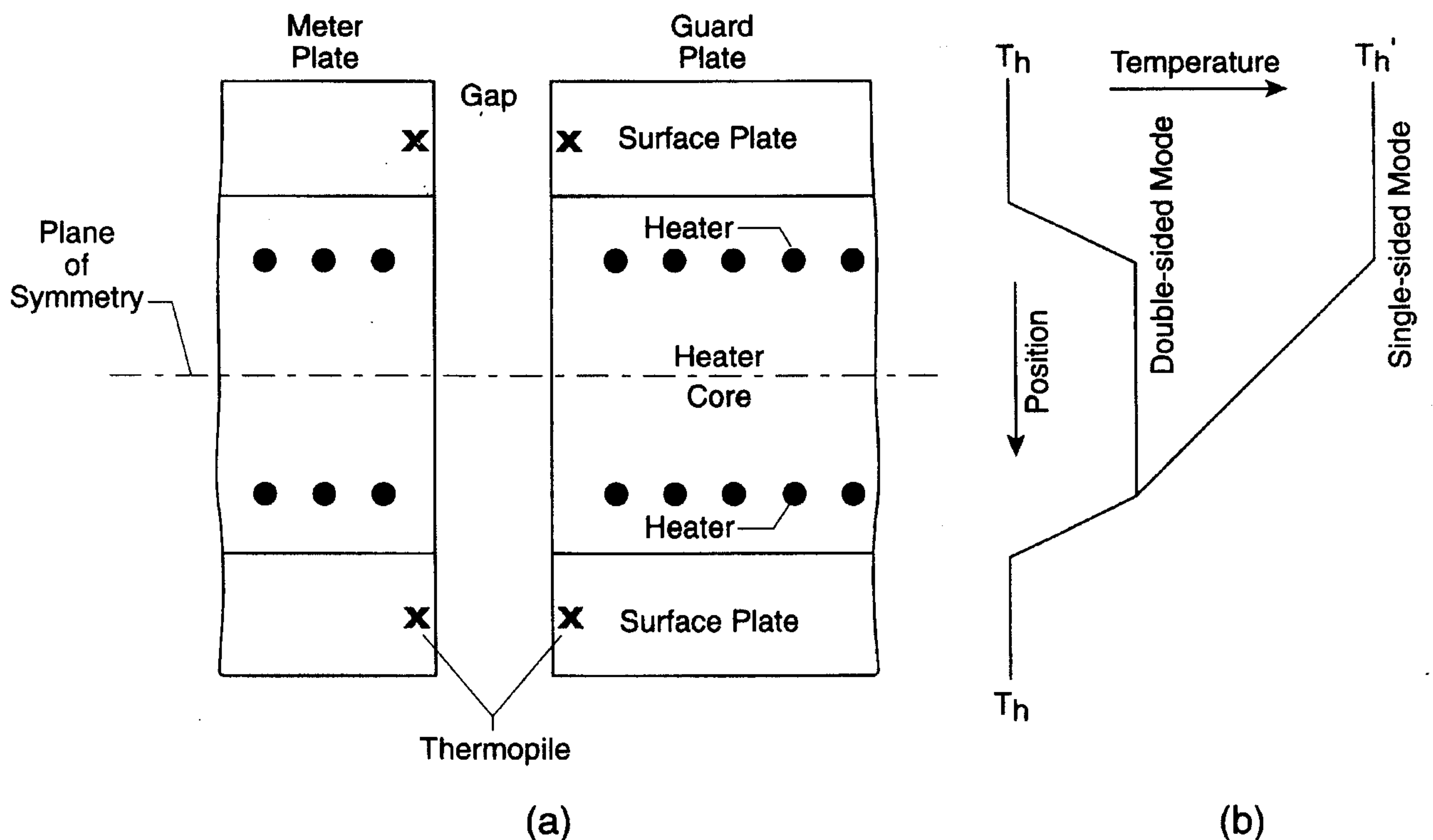
FIG. X2.2 Diagram of (Hypothetical) Guarded-Hot-Plate with Distributed Heat Source, and (b) Corresponding Temperature Profile for Double- and Single-Sided Mode of Operation
