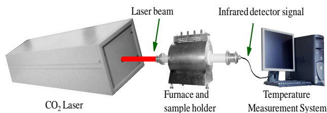
Fig. 1. Thermophysical Properties Measurement Laboratory Experimental Apparatus.
