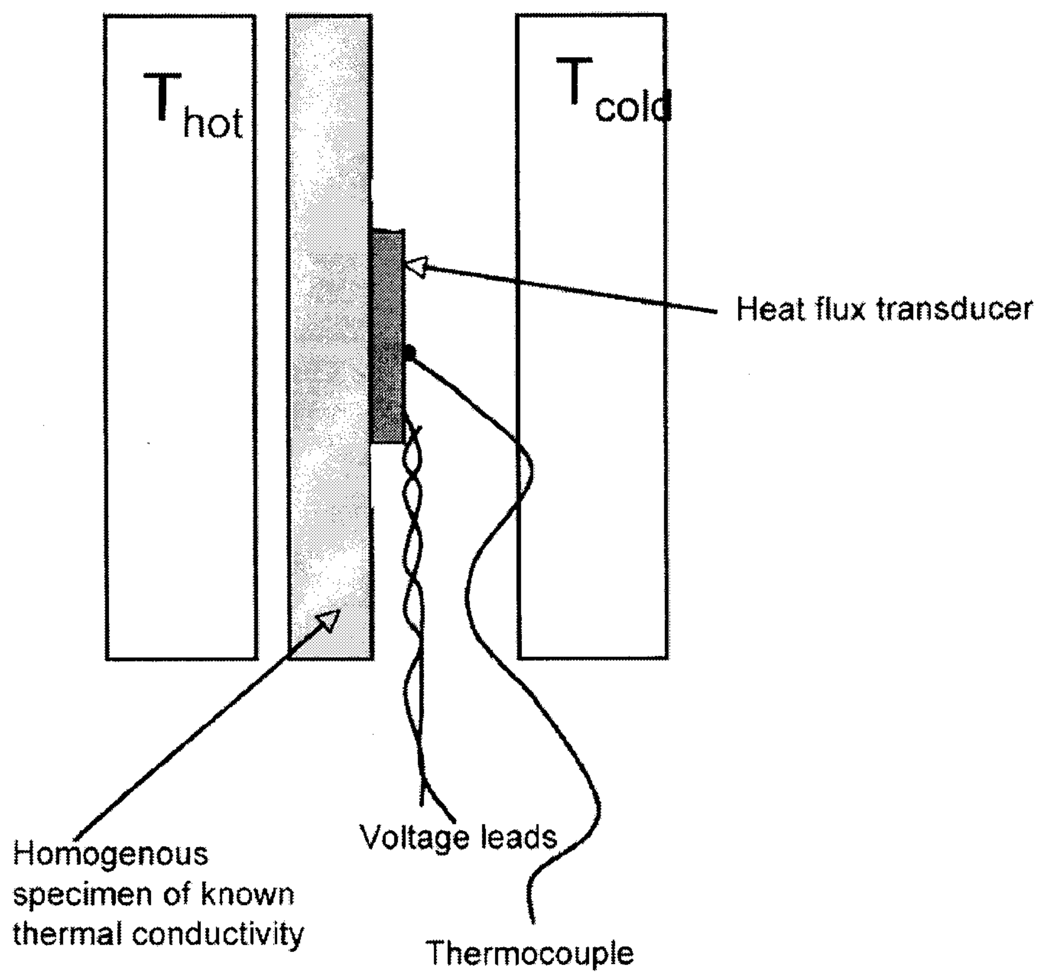
FIG. 3 Example of Test Stack Emulating an Embedded Position Within an Insulated Wall Cavity, Side View
