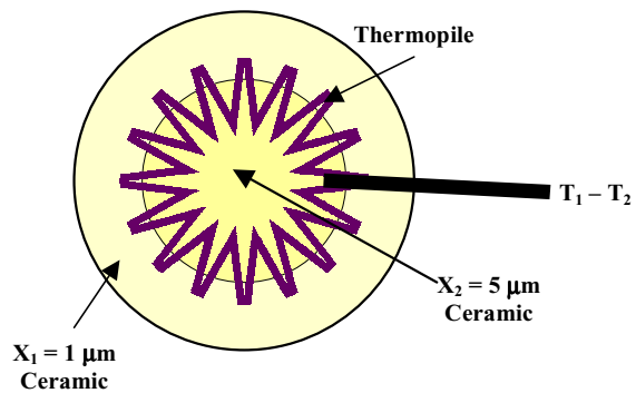
Figure 1: Thermopile-Based Thin Film Heat Flux Sensor (Heat Flux is into the picture).
